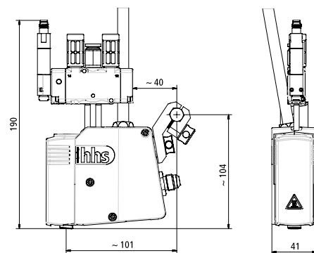
Technical drawing
